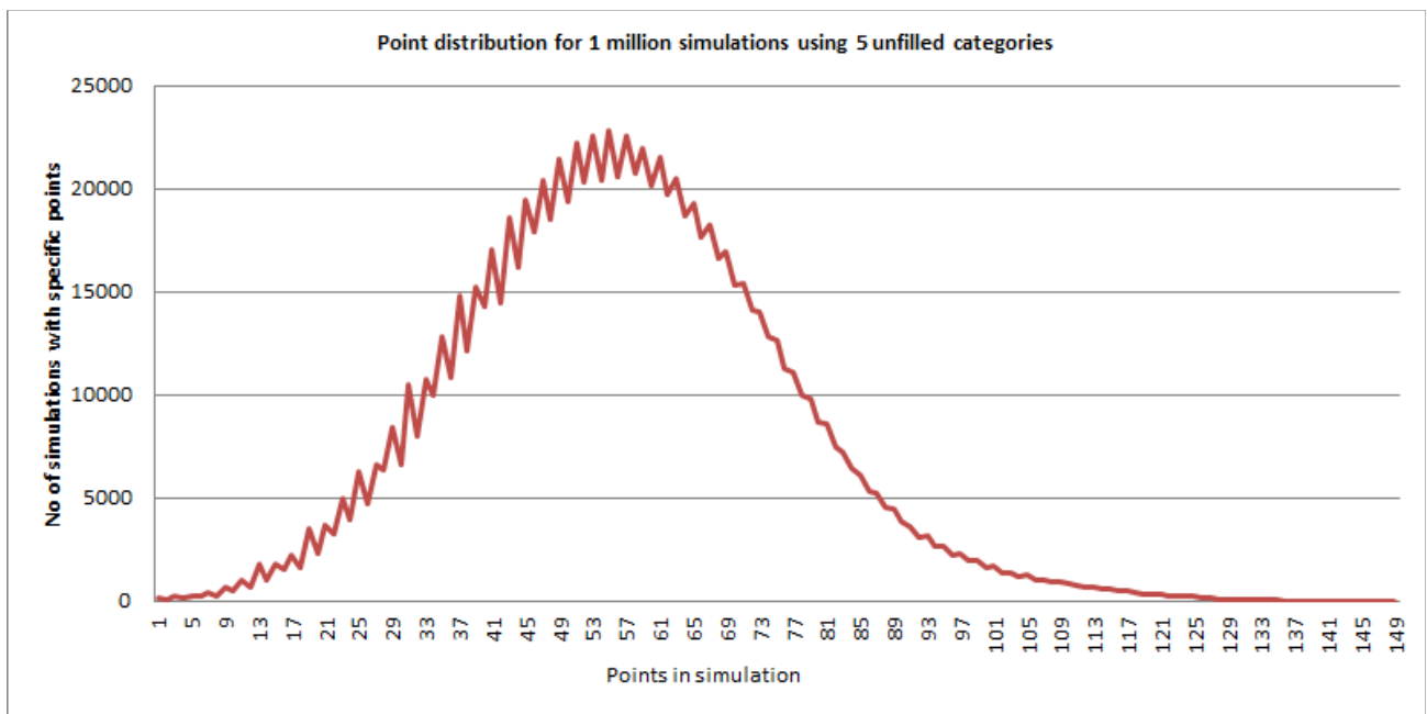
Figure 2. Distribution of points obtained from 1,000,000 simulations starting with five unfilled categories.
