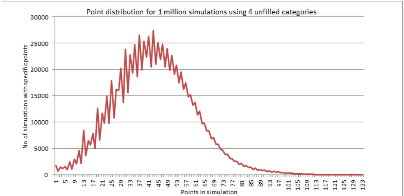
Figure 1. Distribution of points obtained from 1,000,000 simulations starting with four unfilled categories.
