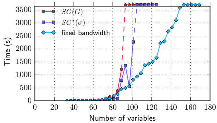
Figure 4: Minisat with fixed variable ordering.
