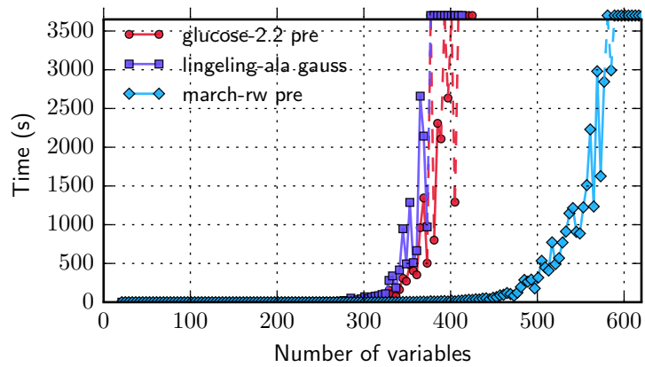
Figure 5: Random 3-CNF formulas.
