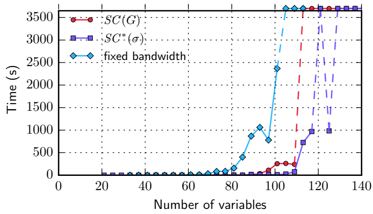
(a) Non-shuffled formulas.
