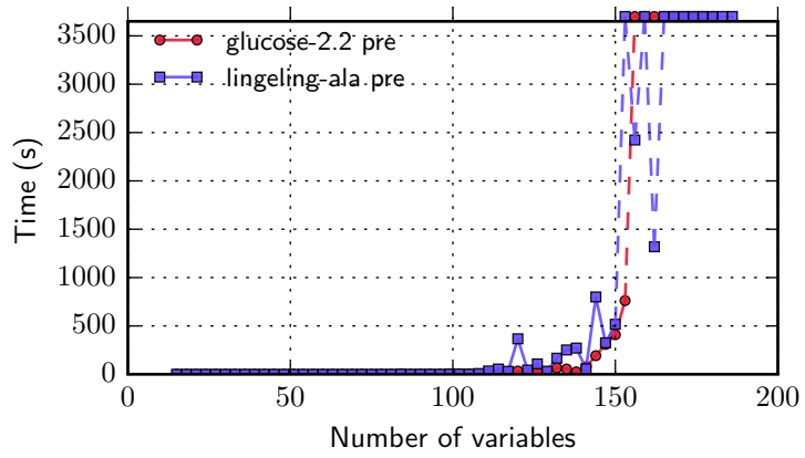
(b) Random assignment of charges to vertices (sum is odd).
