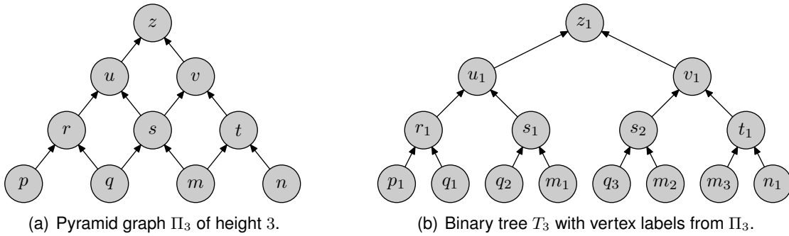
Figure 8: Binary tree with vertices labelled by pyramid graph vertices as in proof of Lemma 8.2.
