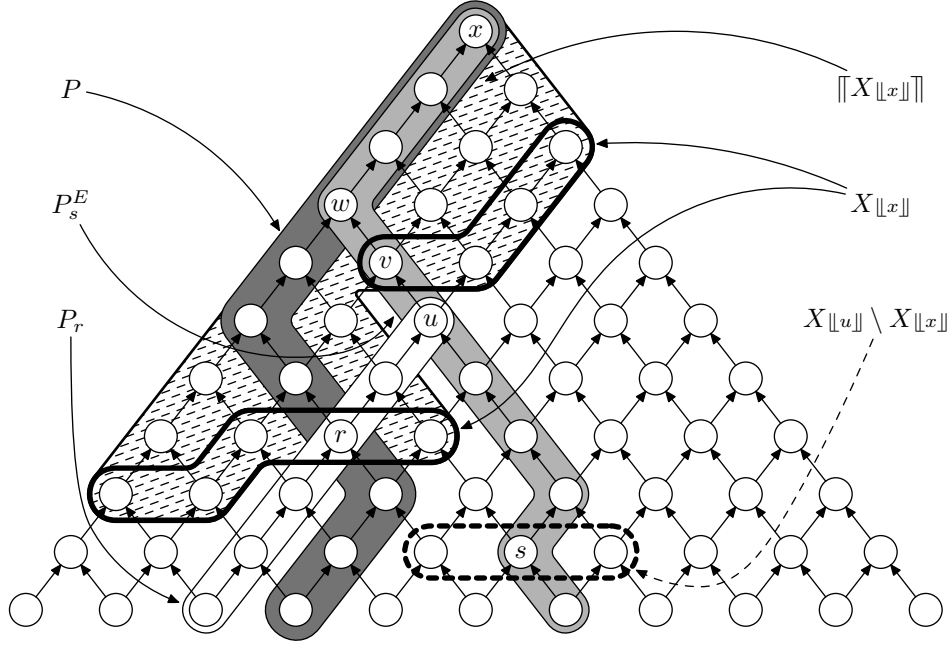
Figure 13: Illustration of proof of Lemma 8.44 that all of X is needed to hide x .
