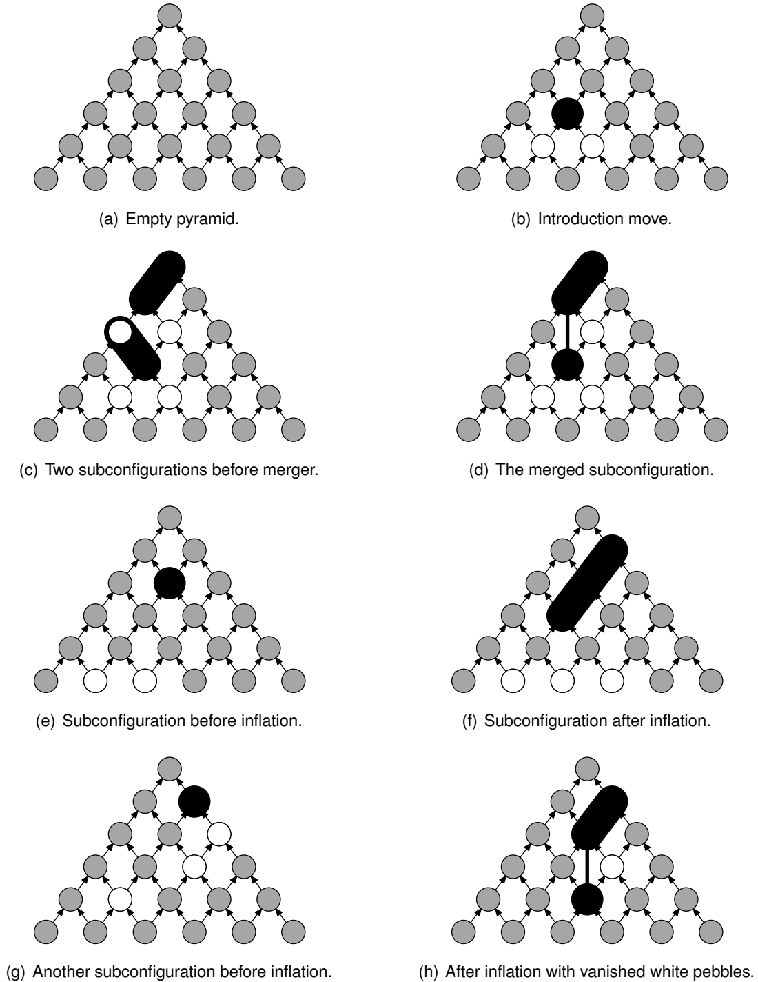
Figure 5: Examples of moves in the blob-pebble game.
