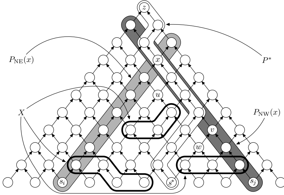
Figure 12: Illustration of proof of Lemma 8.43 that \mathcal{H} is not connected if x \notin \llbracket X \rrbracket .
