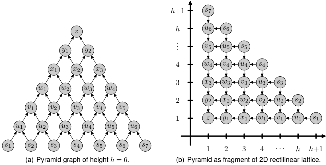
Figure 7: The pyramid \Pi_6 of height 6 with labelled vertices.
