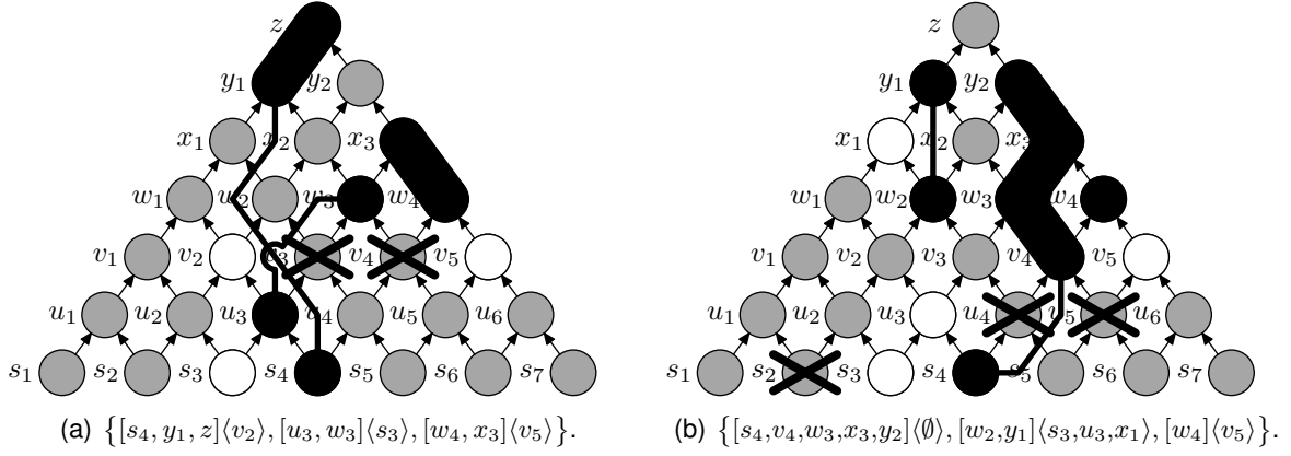
Figure 15: Examples of blob-pebbling configurations with hidden and just blocked blobs.
