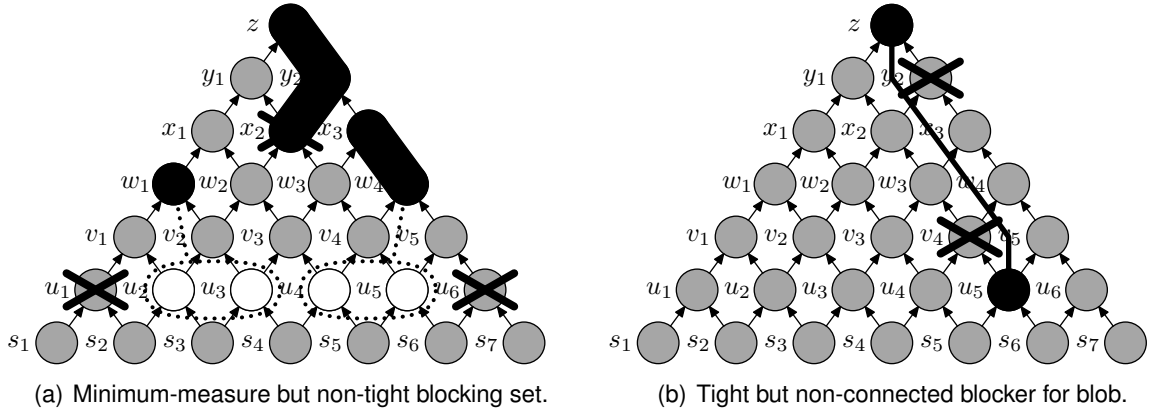
Figure 14: Two blob-pebbling configurations with problematic blocking sets.
