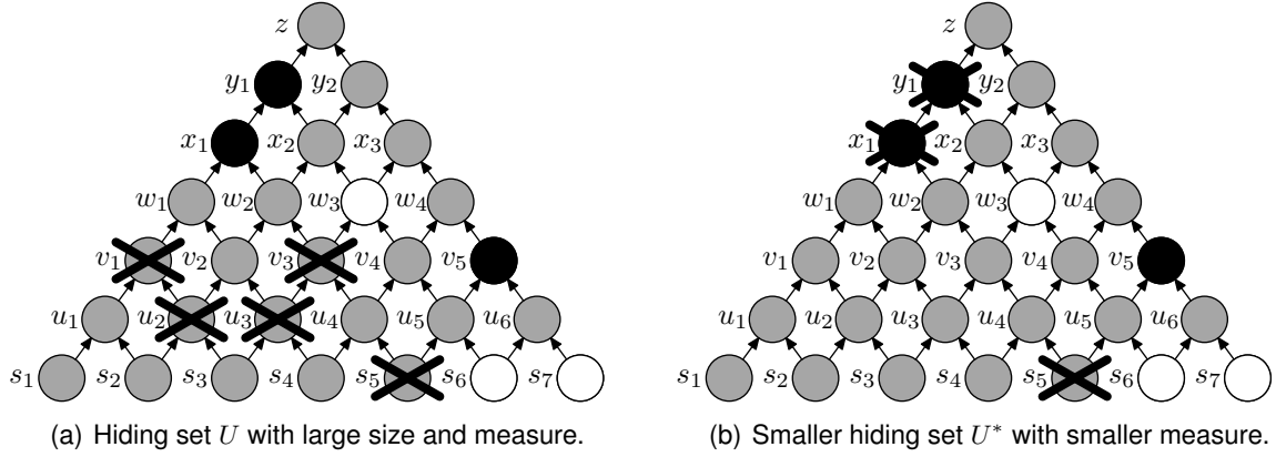
Figure 10: Illustration of hiding sets in Example 8.19 (with vertices in hiding sets cross-marked).
