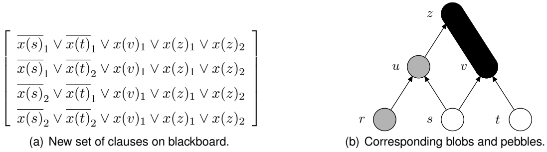
Figure 3: Interpreting sets of clauses as black blobs and white pebbles.
