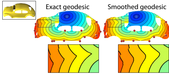
Figure 13: Sharp cusps appear in exact geodesic distances (left) computed for a point on the top of the Beetle (inset). Our framework smooths this field while guaranteeing that all maxima maintain their location and value (right). No new extrema are created.
