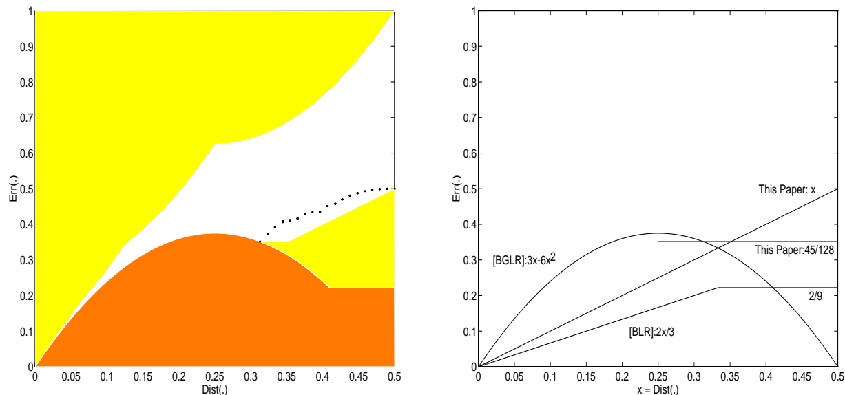
Figure 1: The points (\text{Dist}(f), \text{Err}(f)) in the plane, and the successive lower bounds. See text for discussion.
