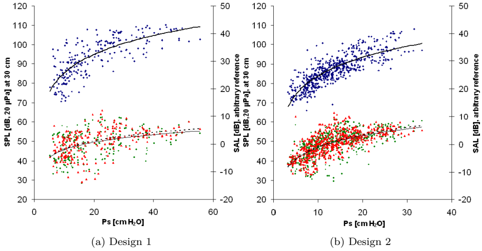
Figure 5.2: Correlations found for SPL and SAL N (measured at the jogular notch) and SAL S according to the division of the dataset of Study II into two statistical designs. The regression outcome for a) Y_{SPL} = 14\ln(x) + 53 , r^2 = 0.5968 and Y_{SALn} = 4\ln(x) - 11 , r^2 = 0.1833 and for b) Y_{SPL} = 13\ln(x) + 52 , r^2 = 0.6732 and Y_{SALn} = 6\ln(x) - 15 , r^2 = 0.4171 . SPL is depicted with blue lozengess, SAL N with green triangles and SAL S with red lozenges. Both SAL measurements clearly demonstrate a weak correlation to P_s . These two figures appear as Figure 5 and 6 in Paper II.
