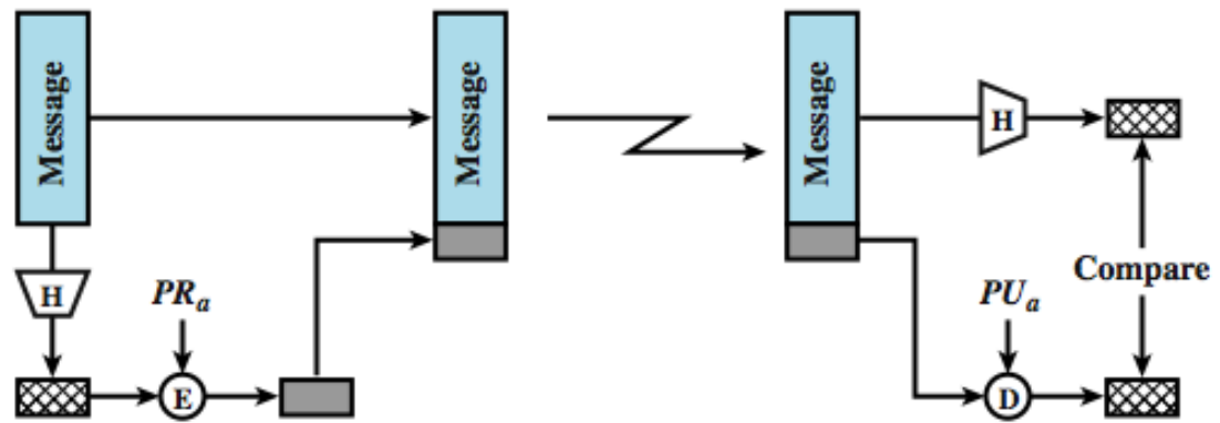
(b) Using public-key encryption
