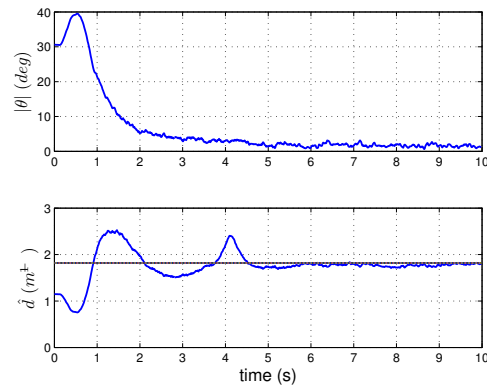
Fig. 6 : Real robot trial. Upper plot: estimation error for motion axis, lower plot: estimated inverse distance between hinge and end-effector. True value (1.82) is marked with a line.
