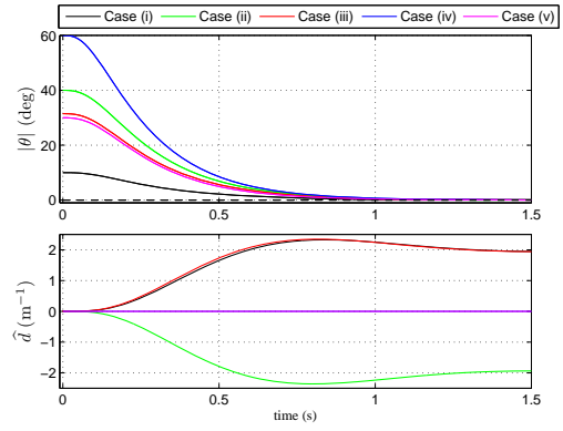
Fig. 3 : Upper figure: estimation error in the orientation of motion axis, lower figure: estimates of the inverse distance between hinge and end-effector. True values are 2 for cases (i) and (iii), -2 for case (ii), and 0 for cases (iv) and (v).
