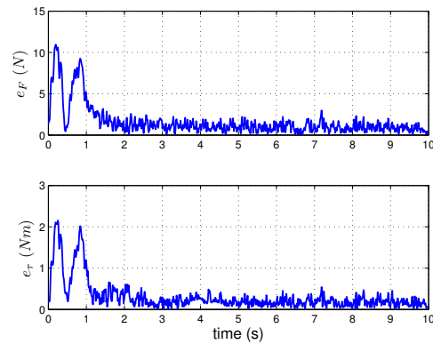
Fig. 7 : Real robot trial. Upper figure: norm of the projected force error, lower figure: norm of the torque error.
