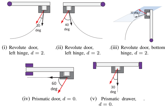
Fig. 2 : The five different simulation cases. The angular measurement indicates the initial error. Note that all scenarios are initialized with the same estimate.
