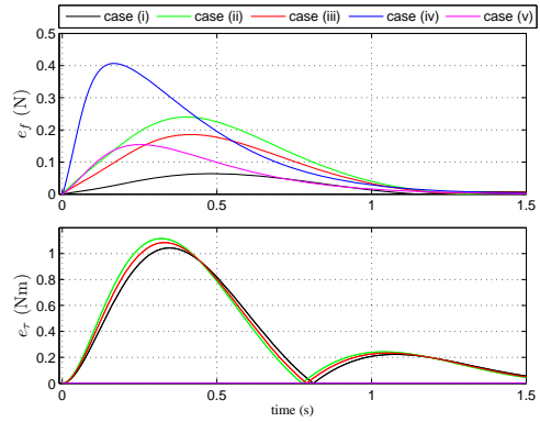
Fig. 4 : Force and torque responses, upper figure: norm of the projected force error, lower figure: norm of the torque error
