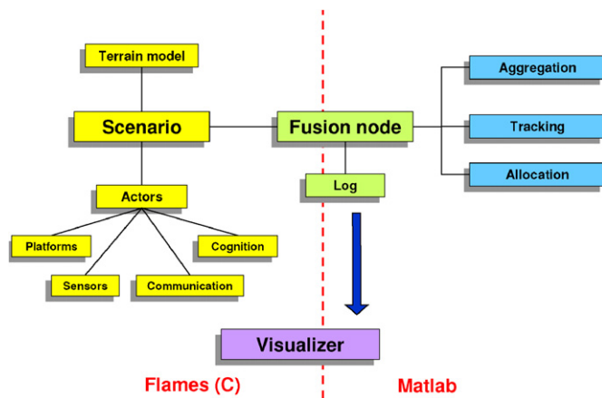
Fig. 10. Connections between different parts of IFD03. Lines between modules mean that the modules exchange data. Note that the Visualizer is a separate program, while all the other modules are linked into the Fire program.
