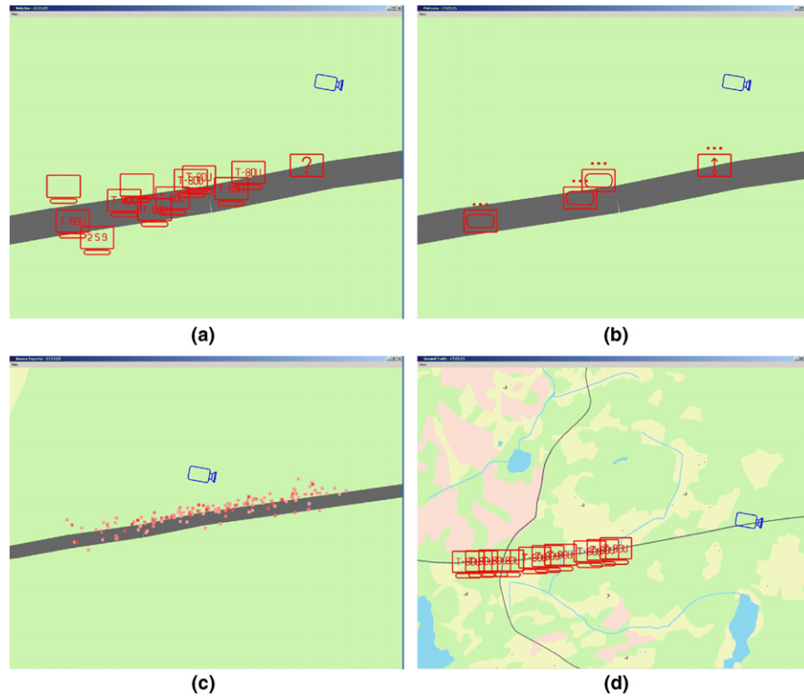
Fig. 15. Aggregation results at the roadside camera. Time is 17:25:25 (hh:mm:ss). Vehicle ground truth and sensor reports views are shown for comparison. (a) Vehicles estimate. (b) Platoons estimate. (c) Sensor reports. Color becomes less saturated as reports are ageing. (d) Vehicle ground truth.
