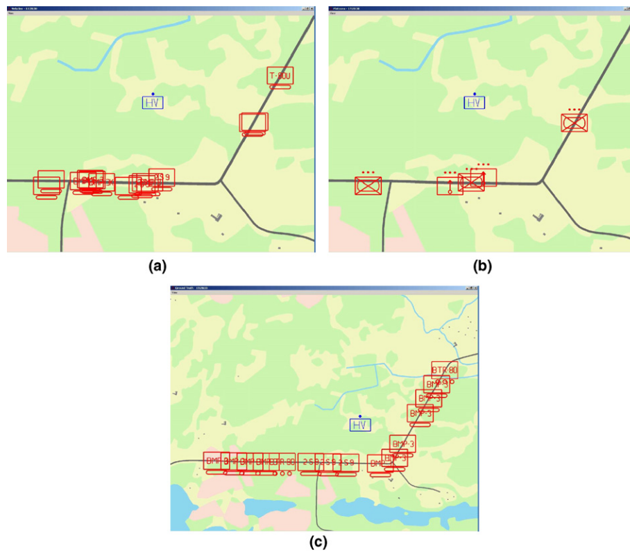
Fig. 16. Aggregation results from Home Guard observations of vehicles on the northern road. Time is 17:28:30. The vehicle ground truth view is shown for comparison. (a) Vehicles estimate. (b) Platoons estimate. (c) Vehicle ground truth.
