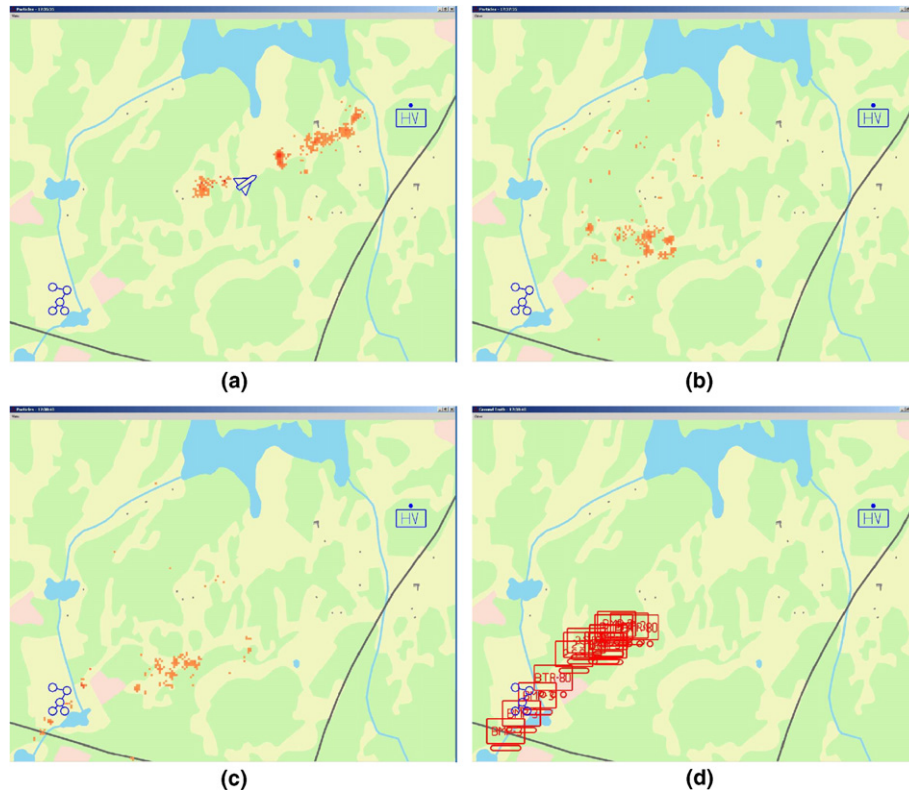
Fig. 18. Results from particle filter tracker during the terrain passage, cf. Fig. 17. Vehicle ground truth at 17:38:40 is shown for comparison. (a) Particle histogram at 17:35:35. (b) Particle histogram at 17:37:35. (c) Particle histogram at 17:38:40. (d) Vehicle ground truth at 17:38:40.
