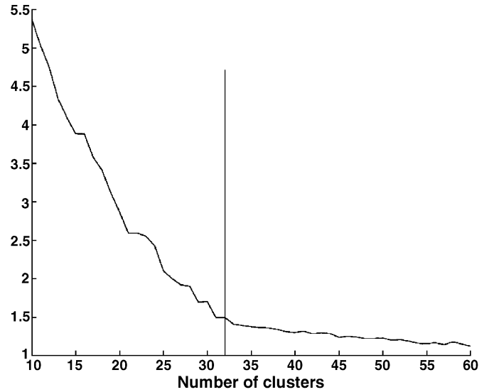
Fig. 6. Logarithm of the total weight of conflict, showing a qualitative change in behavior near the correct number of clusters. The result in this figure is based on clustering all intelligence obtained from sensors observing the advance of one mechanized battalion.
