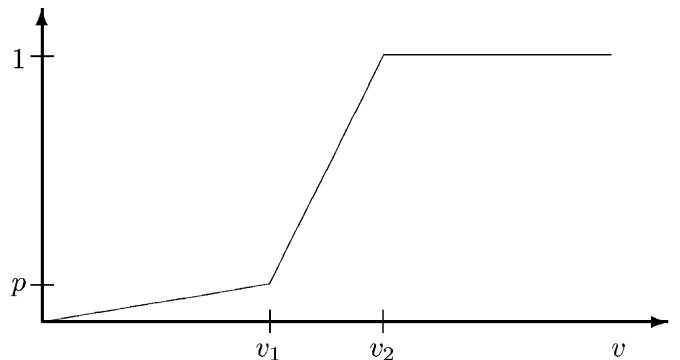
Fig. 4. The relationship between speed and conflict.
