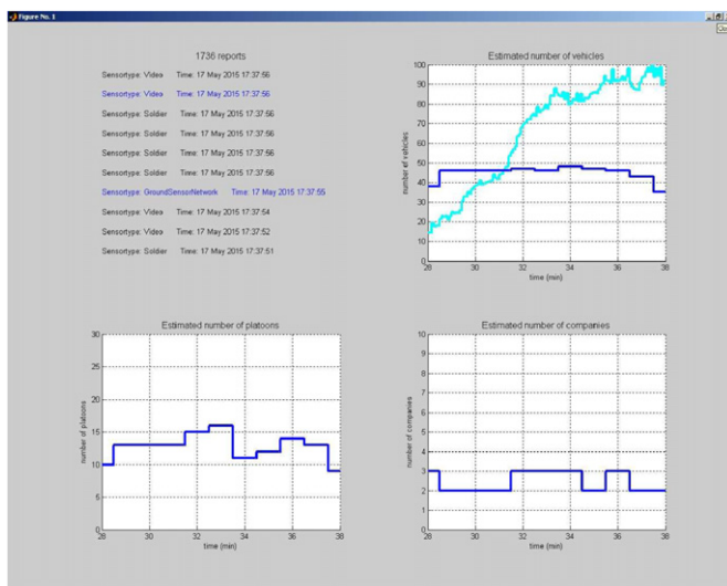
Fig. 12. Snapshot of the standard status view in IFD03. The sub-plots show incoming reports and the estimated number of vehicles, platoons and companies over time.
