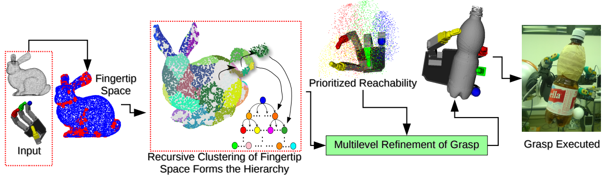
Fig. 1. Given object point cloud and hand model, our system generates a hierarchy of fingertip units (blue) by recursive cluster analysis of the fingertip space . This hierarchy is searched for feasible combinations of contacts with multilevel refinement. The search is prioritized by hand reachability and grasp adaptability measures. Finally, the synthesized grasp is realized by solving inverse kinematics for the selected contacts through optimization.
