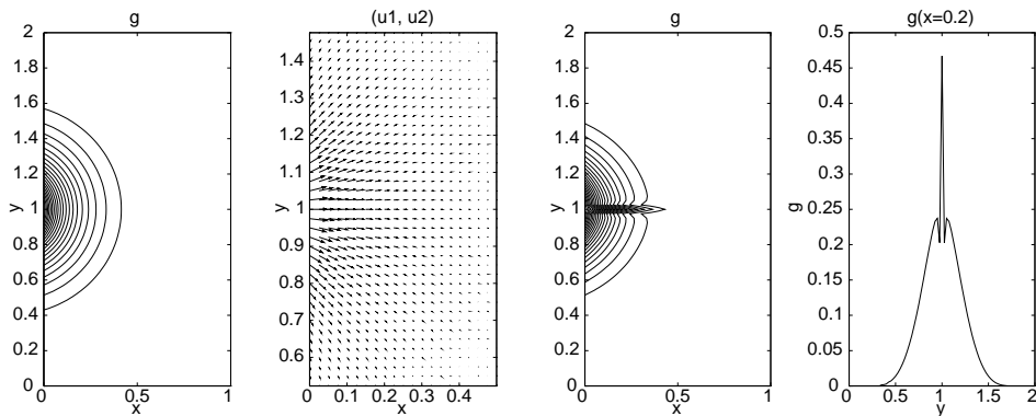
(a) Lax–Friedrichs scheme: contour plot of g (left) and quiver plot of vector field \mathbf{u} = (u_1, u_2) (right)
