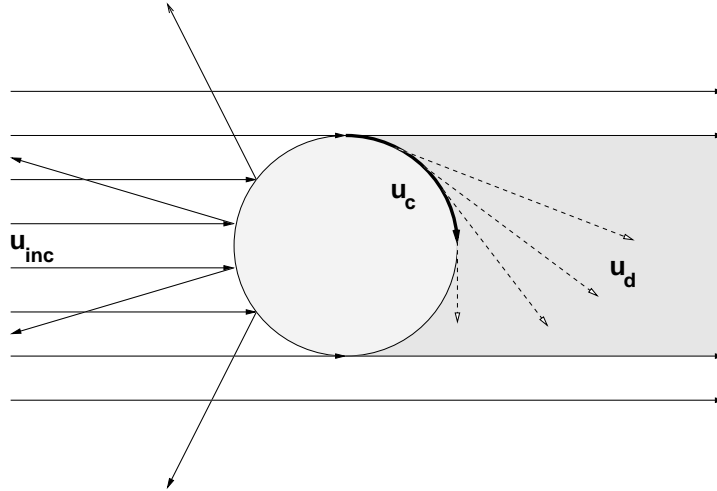
Figure 2.4. Diffraction by a smooth cylinder. The incident field u_{\text{inc}} induces a creeping ray u_c at the north (and south) pole of the cylinder. As the creeping ray propagates along the surface, it continuously emits surface-diffracted rays u_d with exponentially decreasing initial amplitude.
