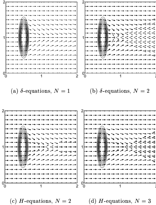
Figure 5.4. Convex lens . Ray angles for \delta - and H -equations with different N . A contour plot of the index of refraction is overlaid on the solution.
