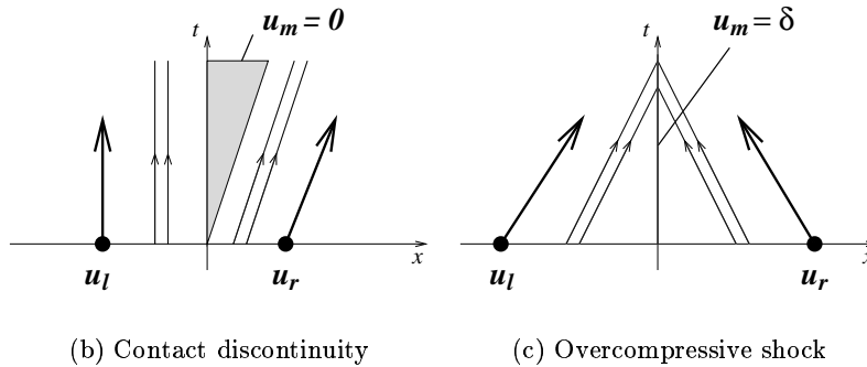
Figure 5.1. The Riemann problem, with Hugoniot loci for the left and right states in phase space and the two different types of discontinuity in (t, \mathbf{x}) space.
