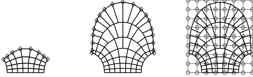
Figure 4.2. Wave front construction. Markers ( \diamond ) on the wave front are propagated as ordinary rays (left). The grid approximates the wave front in physical space, \mathbf{x}(t, r) at constant t - and r -values. When the markers move too wide apart to accurately describe the front, new markers are inserted via interpolation (middle). The travel times and possibly amplitudes on the wave front are interpolated onto a regular grid as the front propagates (right).
